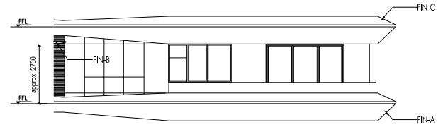
ELEVATION 1 not to scale
